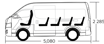
Long Body High Roof (GX)
