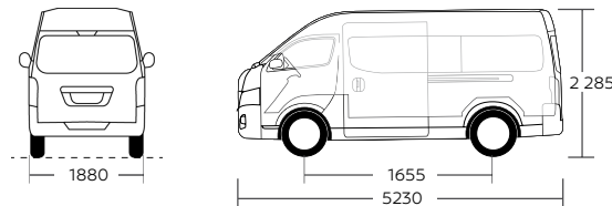
Wide Body, High Roof Wide Long Body, High Roof (FX)
