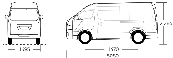
Long Body High Roof (CX)
